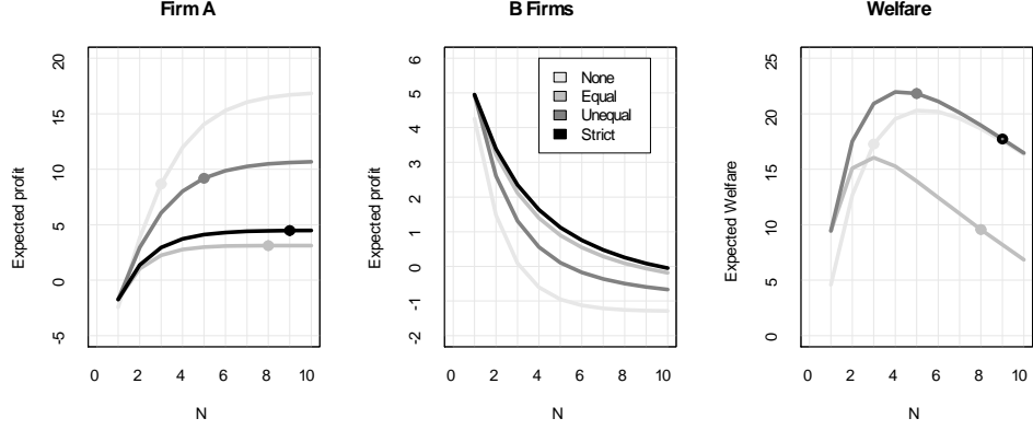
Figure 2: Illustration of a single simulation of model 2, for c_A = 8 , c_B = 1.3 , \sigma = 0.5 and z = 0.75 . The left plot shows expected profits of firm A. The middle plot shows the expected profit of a component B research firm. The right plot shows expected welfare as a function of N and the large dots are the equilibrium welfare levels. Note that the expected welfare curves for an unequal CRO and a strict CRO are identical, but the equilibrium welfare levels are different.
